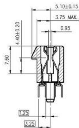
SECTION F-F
