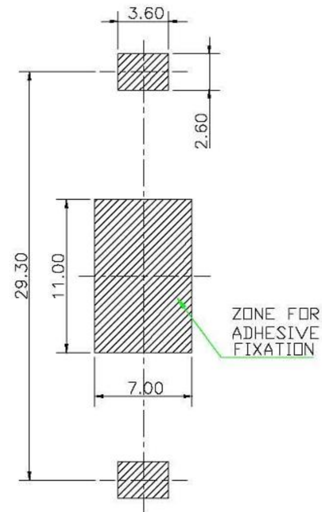
PCB LAYOUT
