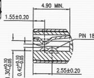
DETAIL C (4 : 1)
