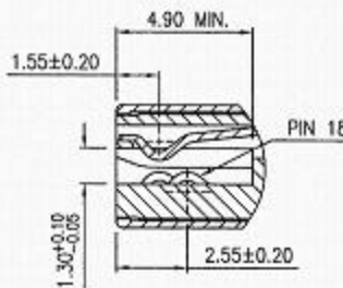
DETAIL C (4 : 1)
